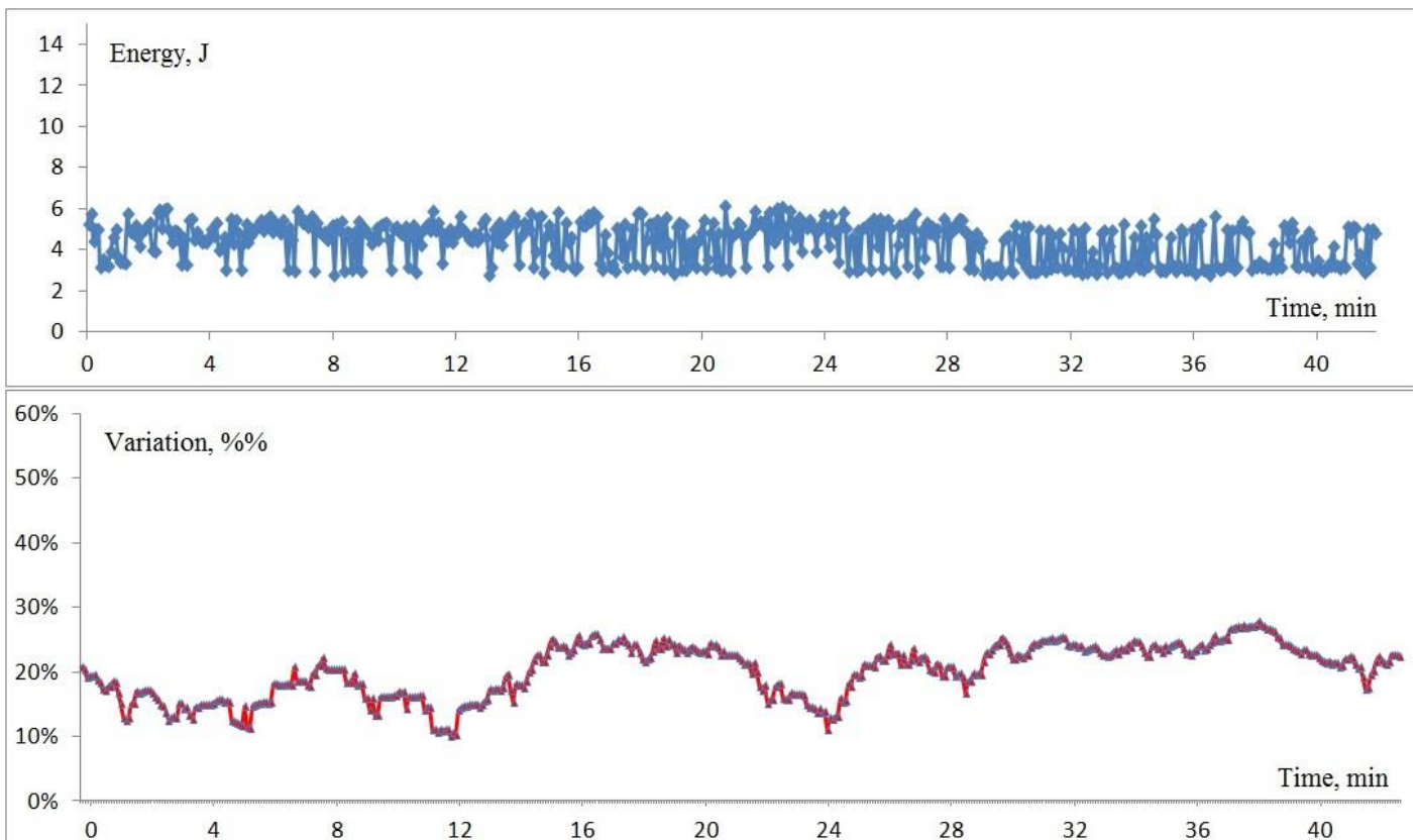
Fig.3. Energy and Variation of a signal recorded by “Sputnik” sensor in a quite place.
