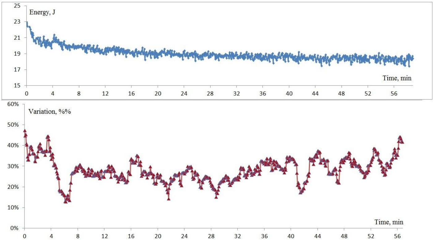
Fig.2. Energy and Variation of a signal recorded by “Sputnik” sensor at the “Vergen de la Perna Ermita” chapel.
